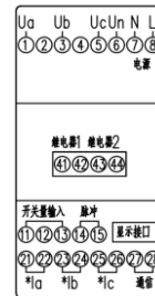
LQZ-100C接线图
